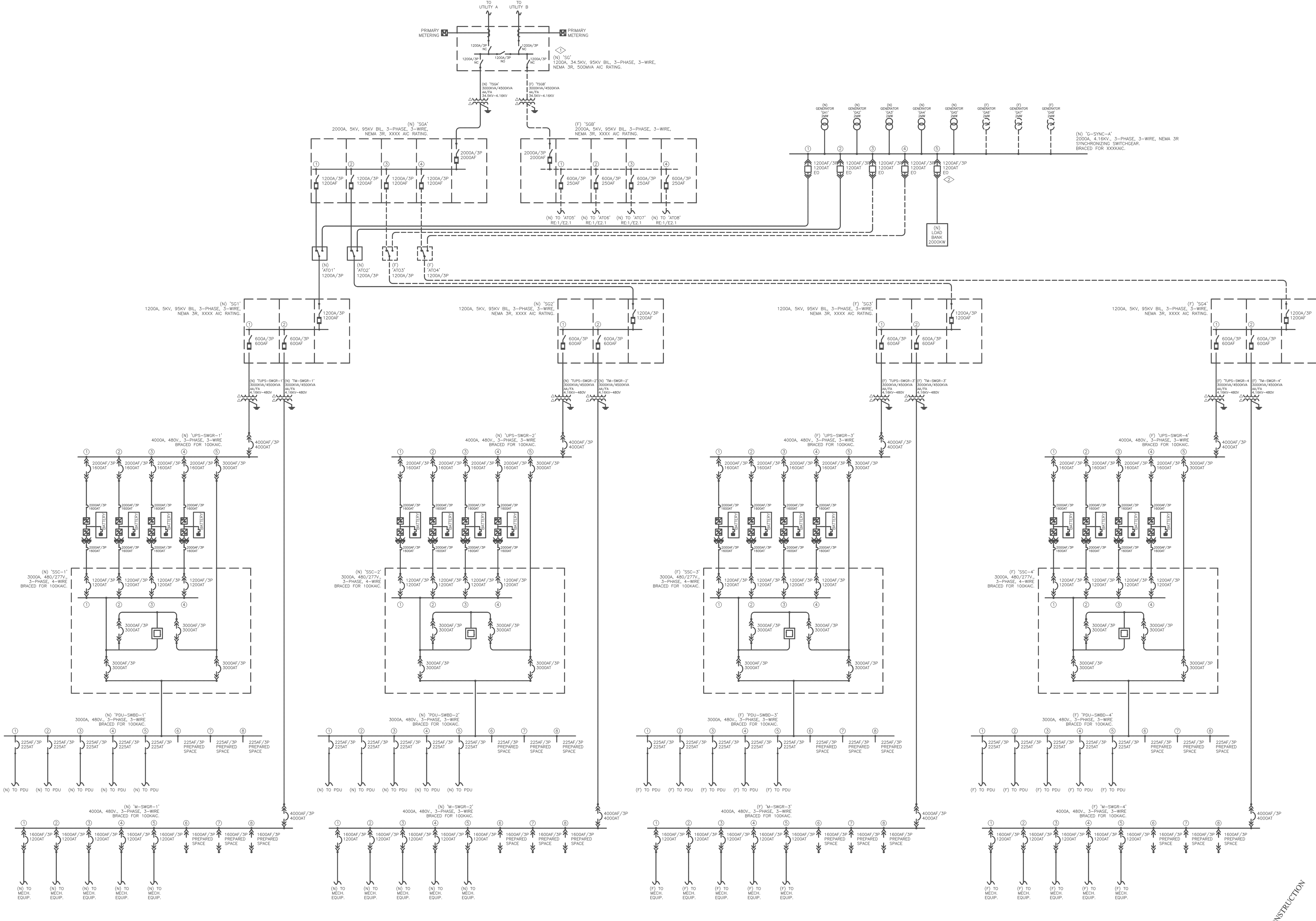
1 ONE-LINE DIAGRAM E2.0 SCALE: NONE
