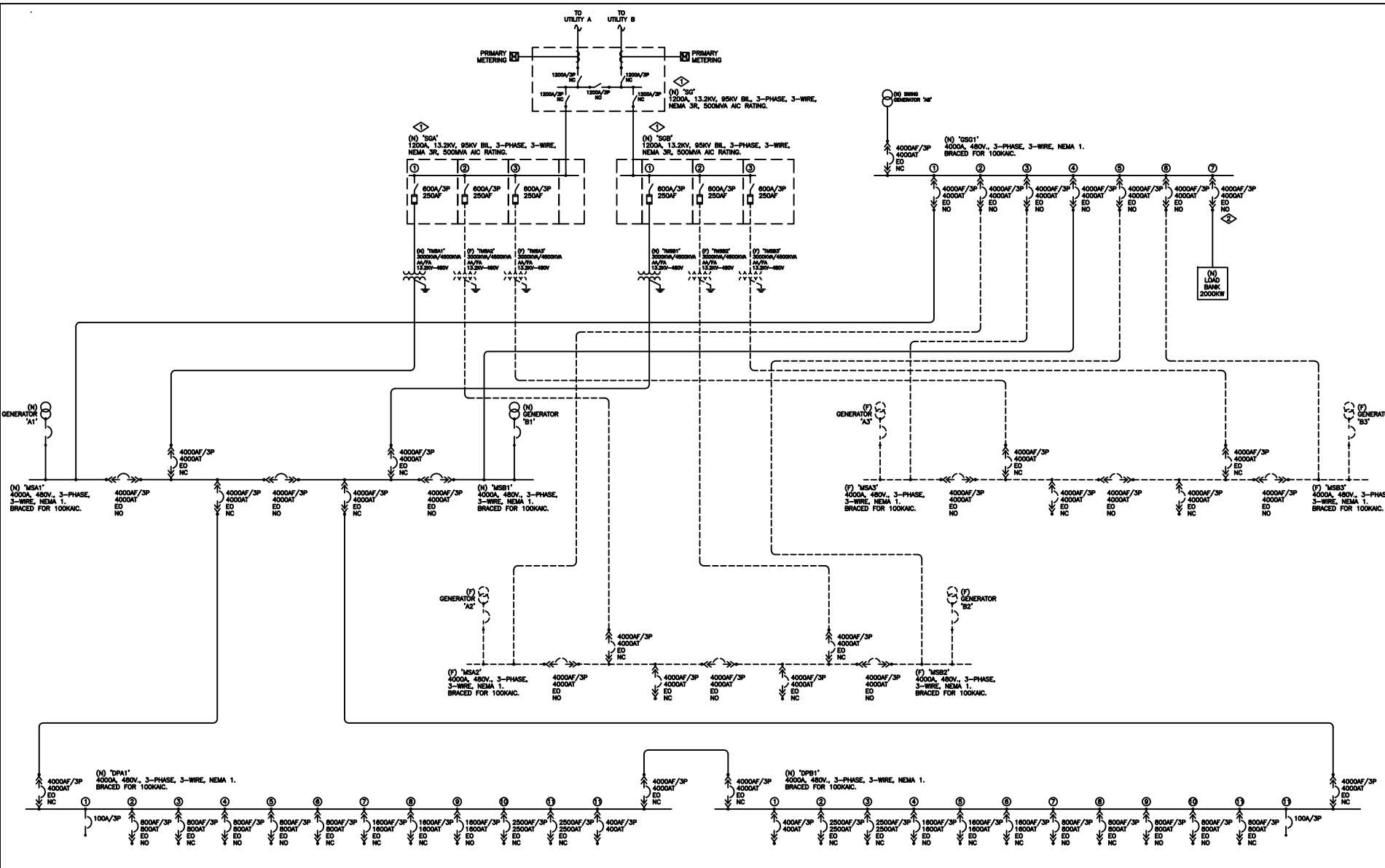
1 ONE-LINE DIAGRAM E2.0 SCALE: NONE
